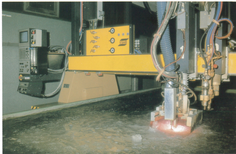
SUPRAREX SXE-P either for oxy-fuel or plasma mode
