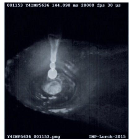
The primary droplet enters the weld pool, and the secondary droplets detach.
