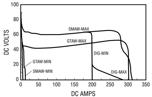
VOLT/AMP CURVE, DC
