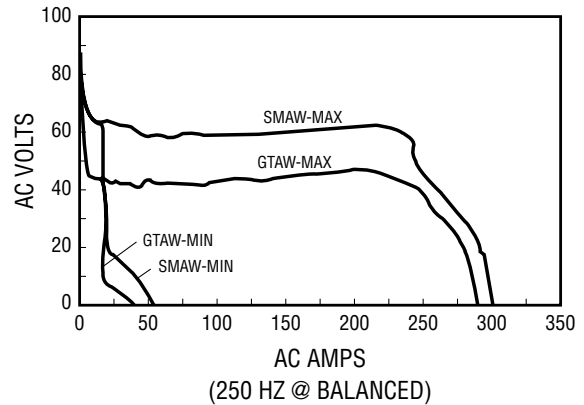
VOLT/AMP CURVE, AC
