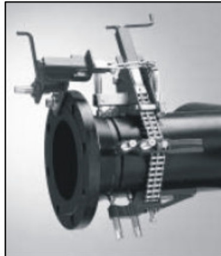
Pipe to Flange
