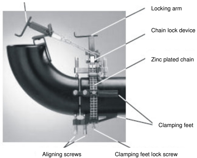
Fitting holder/adjuster
