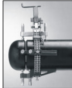
Pipe to End-cap
